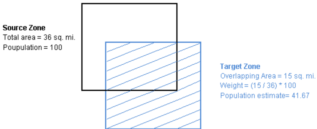
Figure 1. Area-weighted areal interpolation
